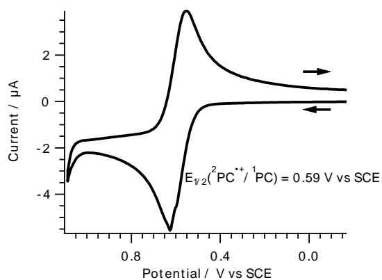
Figure 1: Cyclic voltammetry for 1e - oxidation of ground state 1 PC in DMF with 0.1 M TBAPF 6 at 100 mV/s.
